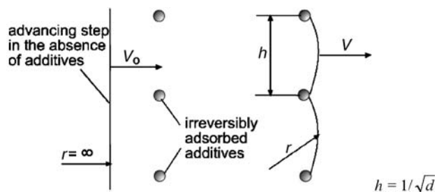
Fig. 2. The crystal growth step in the presence of irreversibly adsorbed additives. V_0 or V is the rate of crystal growth in the absence or presence of irreversibly adsorbed additives.
